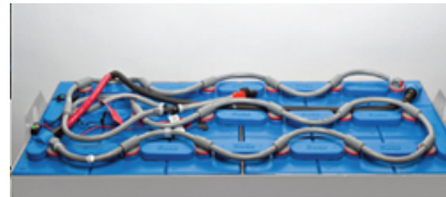
16 Cell Battery Watering System
